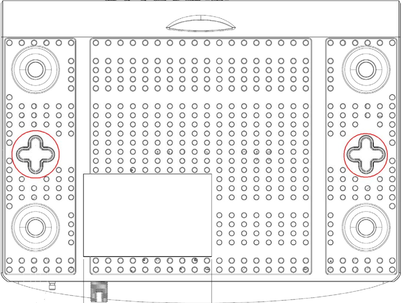
Fig. 1-4 Wall Mounting
