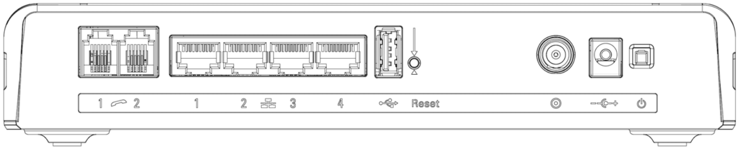
Fig. 1-2 Rear Panel
